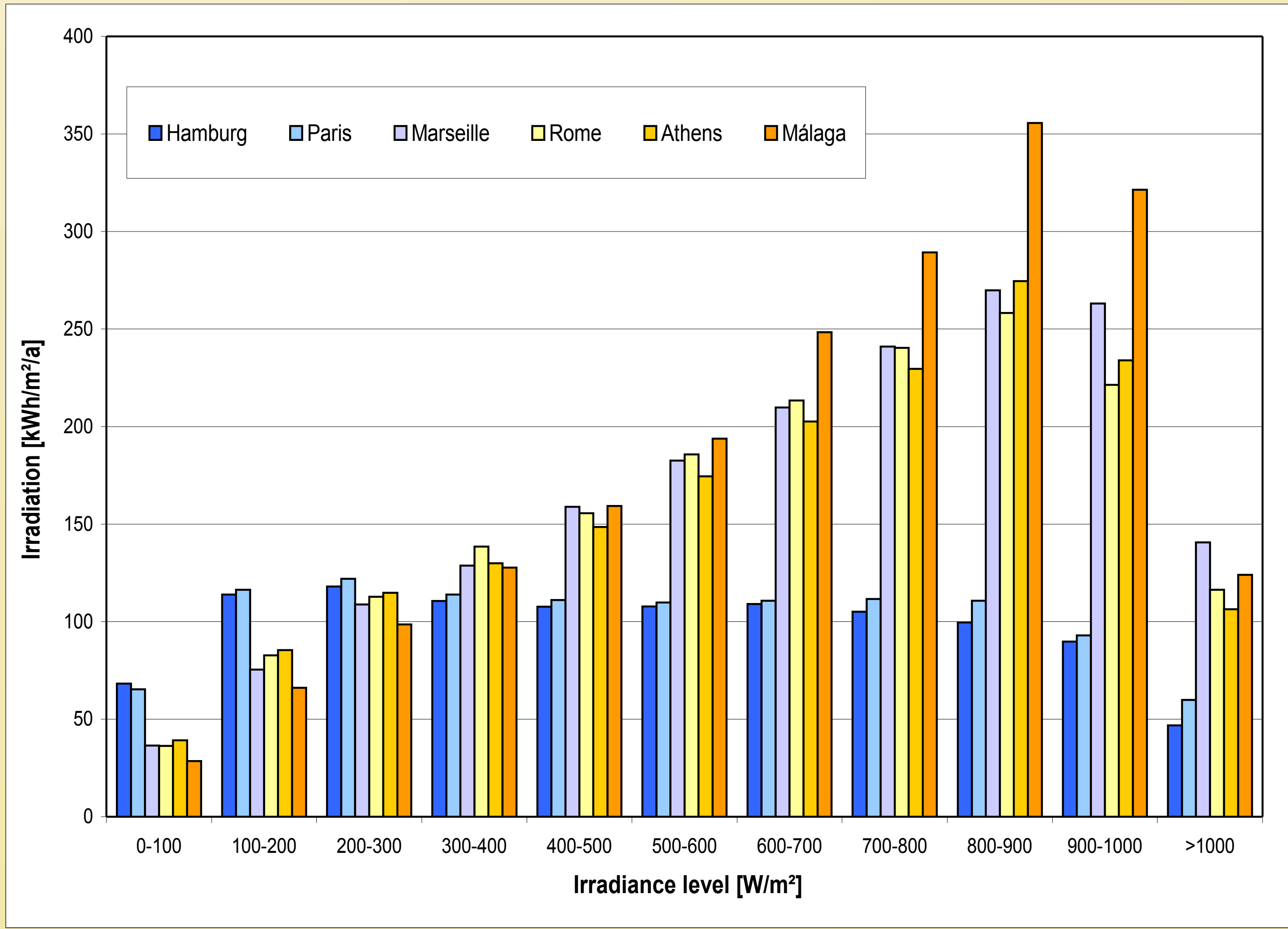
Picture 1: Annual irradiance level distribution for an 30° south inclined plane at different European cities
